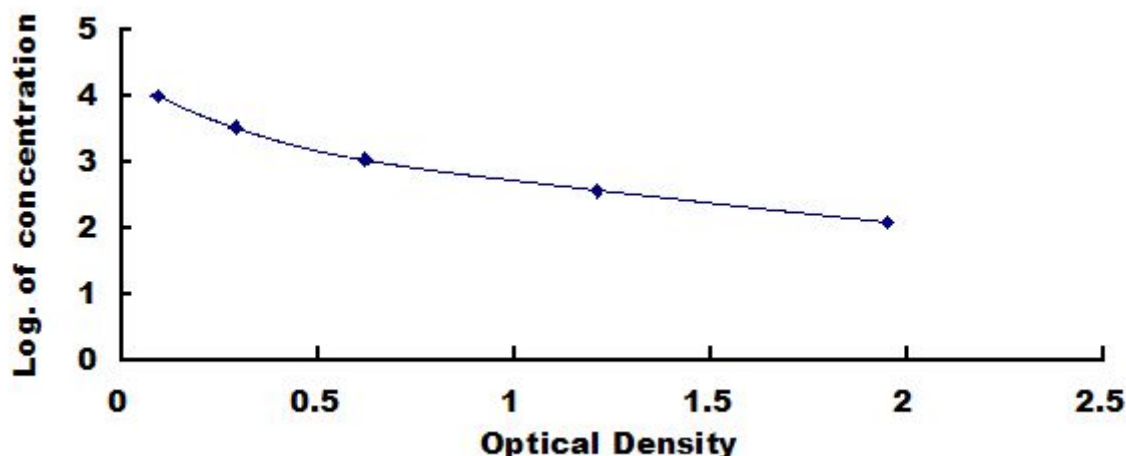
Typical Standard Curve for NT-ProBNP, Rat ELISA.
